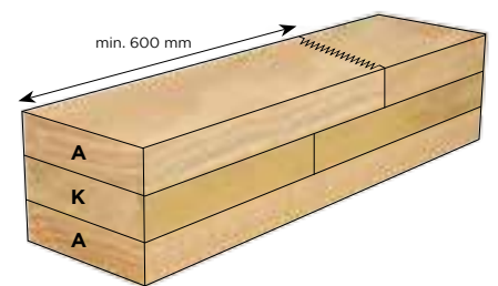
Finger jointed lamella (min 600 mm)
